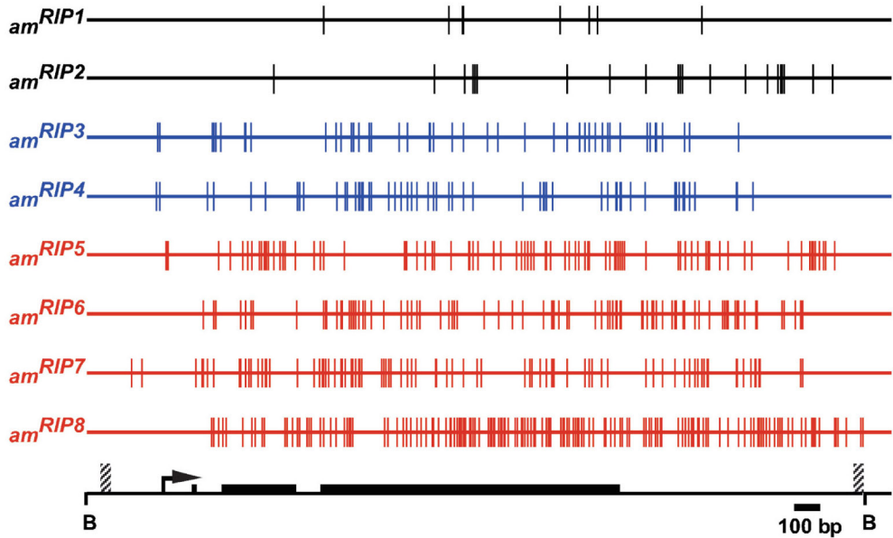
Figure 12. Mutations from RIP and Methylation Status of Eight am Alleles
